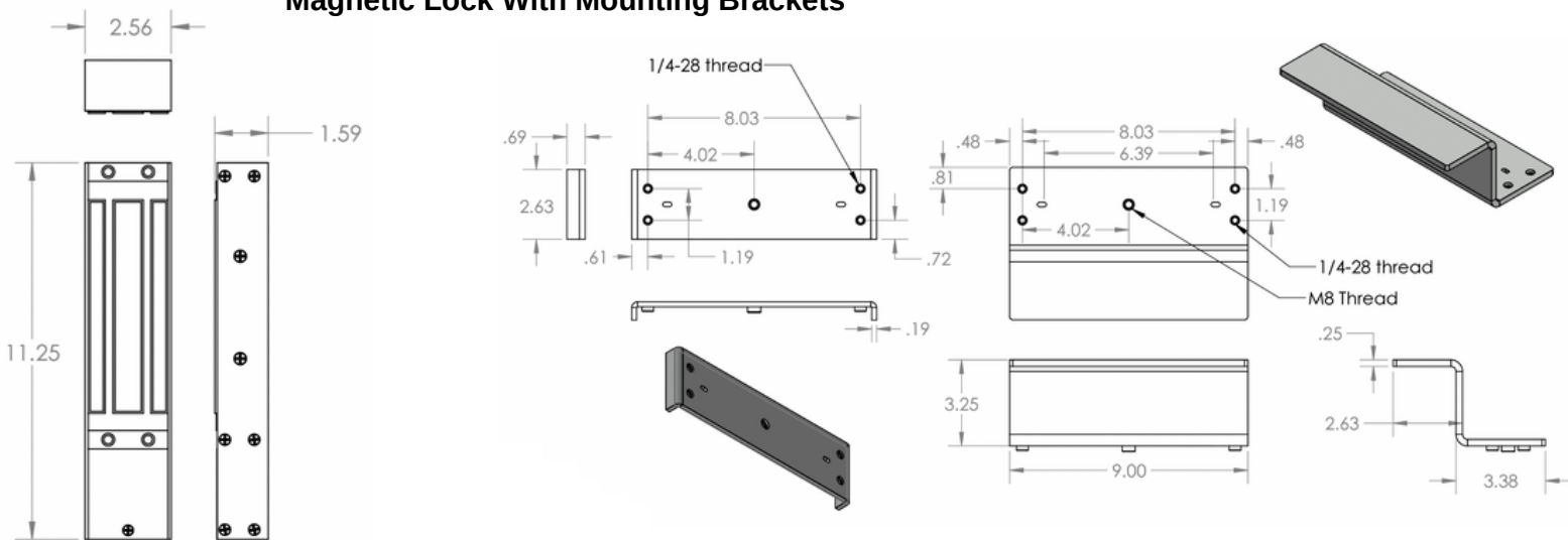
Magnetic Lock With Mounting Brackets
