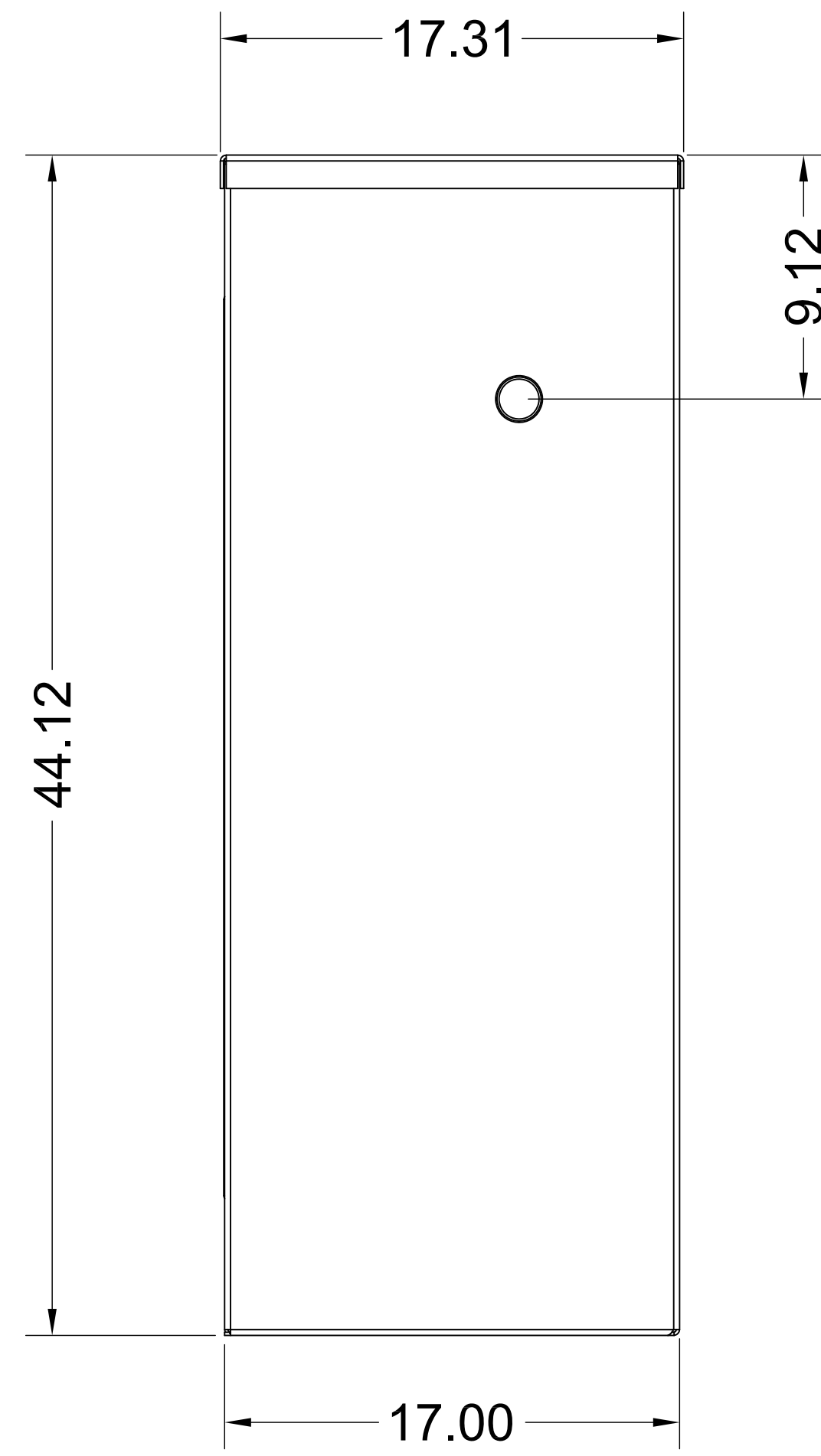
LEFT VIEW
