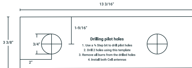
Drilling template diagram
