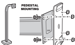
PEDESTAL MOUNTING MOUNT BACKPLATE WITH SECURITY BOLTS AND LOCKNUTS
