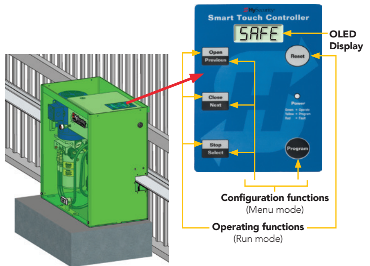
Smart Touch controller keypad
