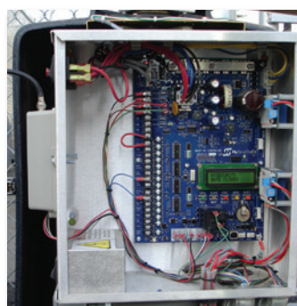
Smart DC Controller in a SwingSmart DC gate operator
