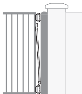
Gate Closed - Front View
