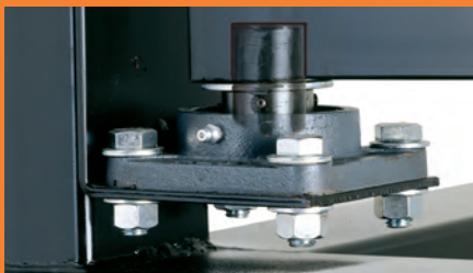
HD FLANGE BEARING HINGE assembly with grease point for heavy wrought iron gates
