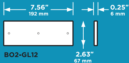
BO1-GL12
